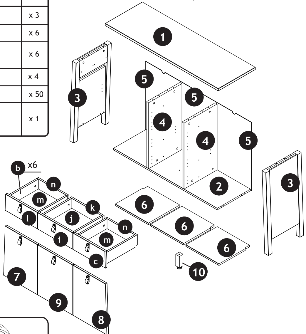
Product Sideboard 125/3+3
